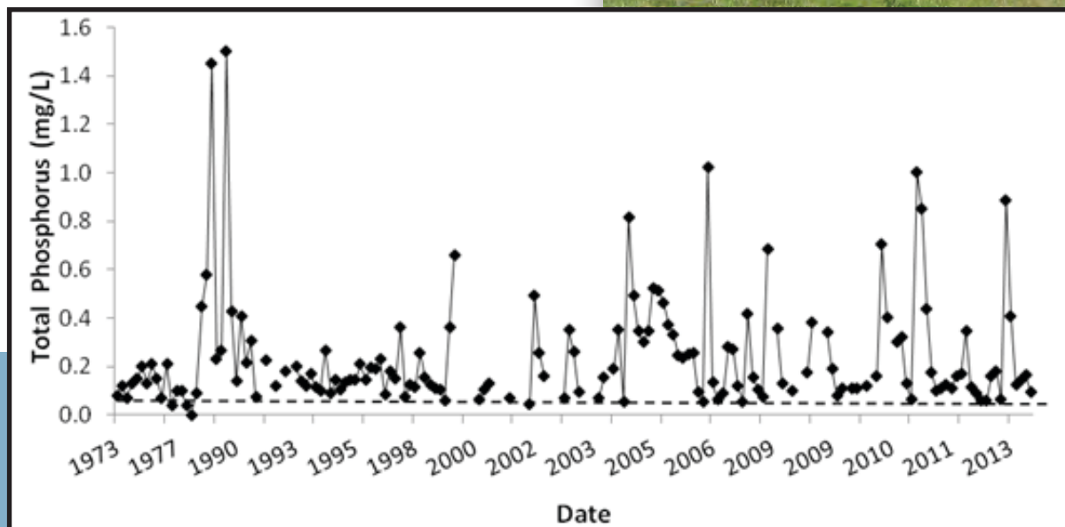
Figure 10: Total Phosphorus concentrations in the Rat River at PR 303 at Otterburne from 1973 to January 2014
